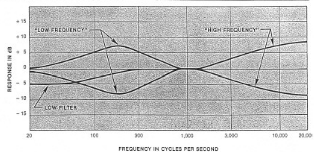
901 IV EQUALIZER CONTROL RESPONSE
