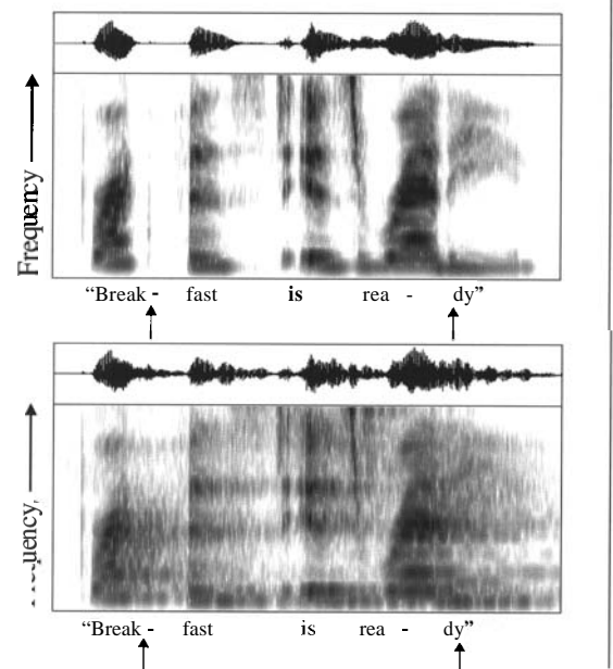
Figure 5. An example of a phrase (“breakfast is ready”) in non-reverberant (upper graph) and in simulated moderately reverberant (lower graph) conditions (RT = 1 second). Each graph shows the time waveform at the top of the panel, and the spectrogram, or change in frequency of the sound over time, at the bottom. Darker patterns indicate more intense sounds; light areas indicate silence or quiet sounds. Note that even with moderate reverberation, many of the temporal patterns of the speech are smeared. The quiet /k/ (shown with an arrow) is apparent in the upper graph but masked in the lower one. The second syllable in “ready” (shown with an arrow) is also masked by the reverberation.
