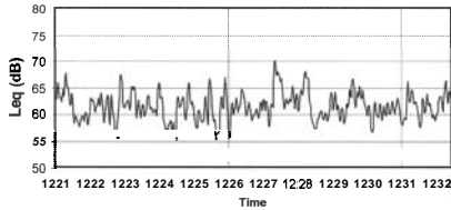
Figure 4a. A typical second-grade class is shown. The 17 students are working quietly and independently, and the teacher is roaming throughout the room, assisting students. A time trace from the sound level meter shows the level of sound occurring over a 10-minute period. The trace shows a background noise level ranging from 59 to 62 dBA that apparently arises from the steady output of the HVAC system. The teacher's voice is measured at 60–62 dBA, resulting in a signal-to-noise (SNR) ratio of 0 dB. At that SNR, we can expect that children of this age are missing significant portions of the teacher's message.
